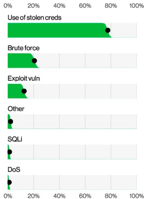
Figure 41. Top Hacking actions in Basic Web Application Attacks breaches (n=713)
